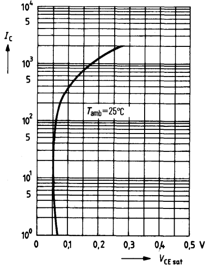
Collector emitter saturation voltage V_{CEsat} = f(I_C) \beta_{FE} = 10; T_{amb} = 25^\circ\text{C}
