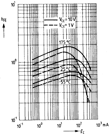
DC current gain h_{FE} = f(I_C) V_{CE} = 1V, V_{CE} = 10V; T_{amb} = 25^\circ C
