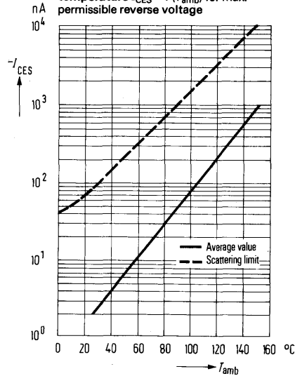
Collector cutoff current versus temperature I_{CES} = f(T_{\text{amb}}) for max. permissible reverse voltage
