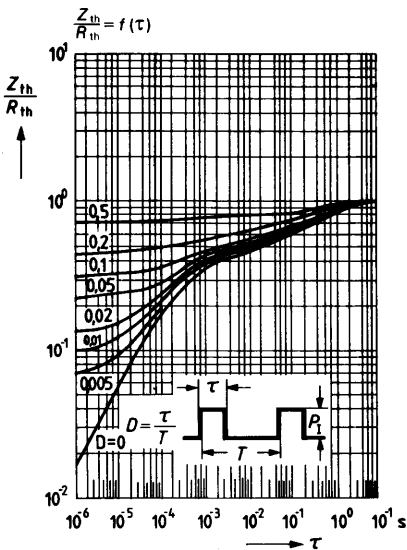
Total perm. power dissipation
