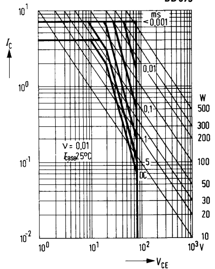
Permissible operating range I_C = f(V_{CE}); v = 0.01; T_{case} = 25^\circ\text{C}
