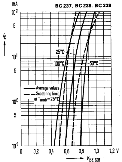
Base-emitter saturation voltage V_{BEsat} = f(I_C); T_{amb} = \text{parameter}; h_{FE} = 20 (common emitter configuration)
