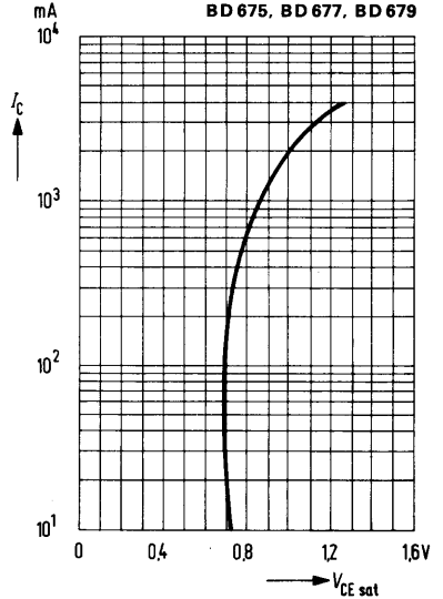
Collector-emitter saturation voltage V_{CEsat} = f(I_C); h_{FE} = 100; T_{case} = 25^\circ\text{C} BD 675, BD 677, BD 679
