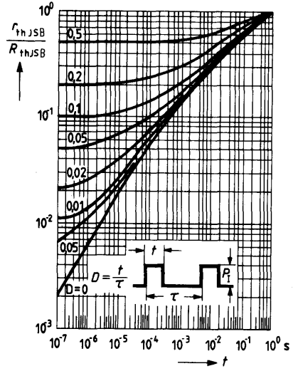
Pulse resistance \frac{r_{\text{thJSB}}}{R_{\text{thJSB}}} = f(t) D = \text{parameter}
