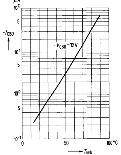
Collector cutoff current versus temperature I_{CBO} = f(T_{amb}) -V_{CBO} = 12\text{ V}
