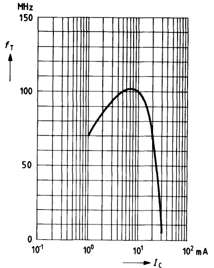
Transition frequency f_T = f(I_C) V_{CE} = 10\text{ V} ; T_{case} = 25^\circ\text{C}
