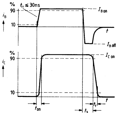
Timing diagram
