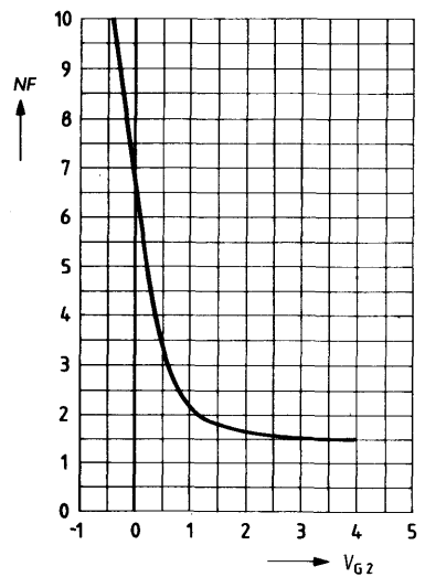
Noise figure NF = f(V_{G2S}) V_{DS} = 15\text{ V} ; V_{G1S} = 0 I_{DSS} = 10\text{ mA} ; f = 200\text{ MHz} R_S = 0\Omega (see figure 1)
