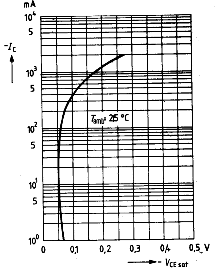
Collector-emitter saturation voltage V_{CEsat} = f(I_C) h_{FE} = 10; T_{amb} = 25^\circ C
