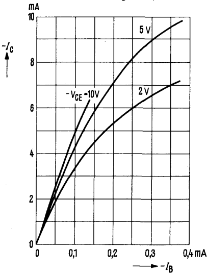
Collector current I_C = f(V_B) V_{CE} = \text{parameter} (common emitter configuration)
