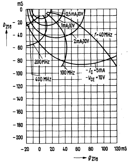
Small signal short circuit forward transfer admittance Y_{21e} (common emitter configuration)
