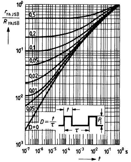
Pulse resistance \frac{r_{thJSB}}{R_{thJSB}} = f(t) D = \text{parameter}
