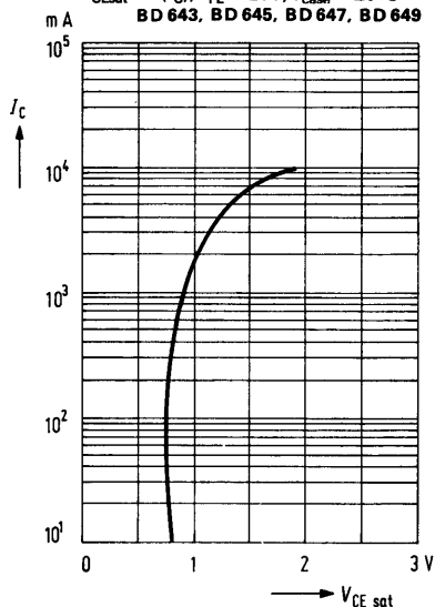
Collector-emitter saturation voltage V_{CEsat} = f(I_C); h_{FE} = 250; T_{case} = 25^\circ\text{C} BD 643, BD 645, BD 647, BD 649
