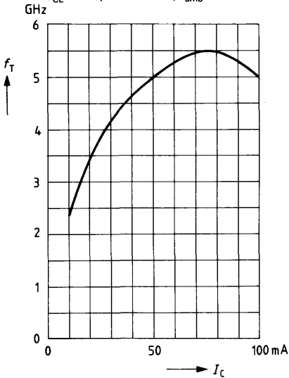
Transition frequency f_T = f(I_C) V_{CE} = 10 V, f = 500 MHz, T_{amb} = 25^{\circ}C
