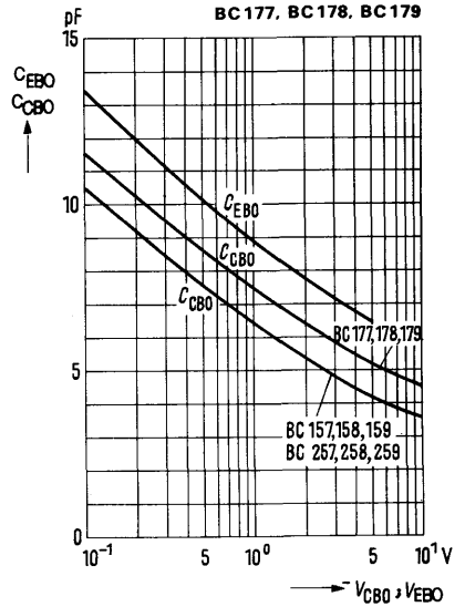
Collector base capacitance C_{CBO} = f(V_{CBO}) Emitter base capacitance C_{EBO} = f(V_{EBO}) f = 1\text{ MHz}; T_{amb} = 25^\circ\text{C}
