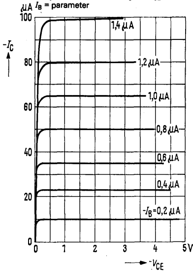
Output characteristics I_C = f(V_{CE})
