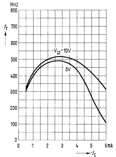
Transition frequency f_T = f(I_C) -V_{CE} = parameter; f = 100 MHz
