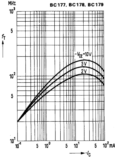
Transition frequency f_T = f(f_C); (T_{amb} = 25^\circ\text{C})
