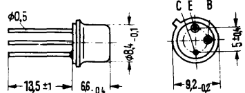
Approx. weight 1.5 g Dimensions in mm
