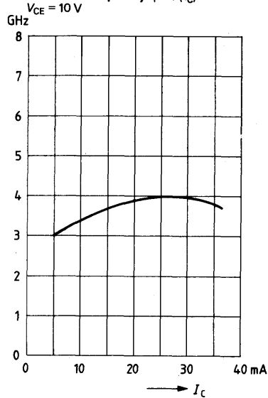
Transition frequency f_T = f(I_C)
