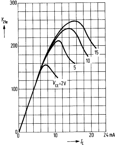
Small-signal short-circuit forward transfer admittance |y_{21e}| = f(I_C)
