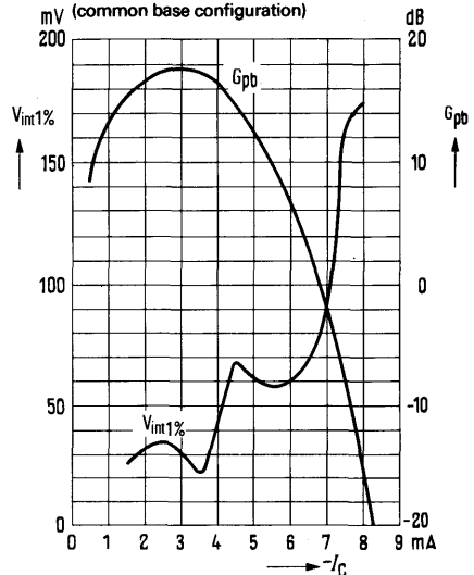
Interference voltage V_{int} 1\% = f(I_C) Power gain G_{pb} = f(I_C) f = 200 \text{ MHz}; -V_{batt} = 12 \text{ V} R_p = 1 \text{ k}\Omega; R_L = 0.9 \text{ k}\Omega (common base configuration)
