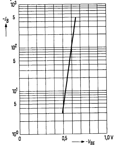
Input characteristic I_B = f(V_{BE}) V_{CE} = 5 \text{ V} ; T_{amb} = 25^{\circ}\text{C}
