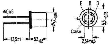
Approx. weight 0.4 g
