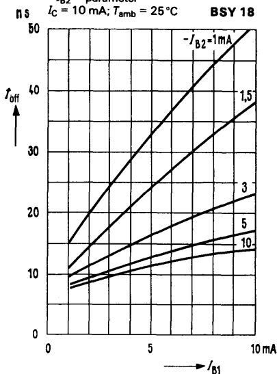
Turn-off time t_{off} = f(I_{B1}) -I_{B2} = \text{parameter}
