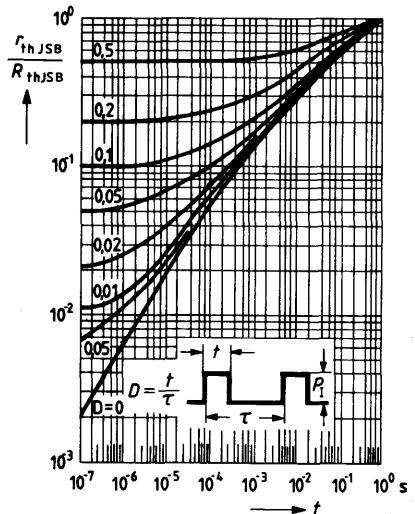
Permissible pulse load \frac{r_{thJSB}}{R_{thJSB}} = f(t) D = parameter
