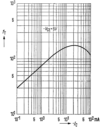
Transition frequency f_T = f(I_C) f_T T_{amb} = 25^\circ\text{C}
