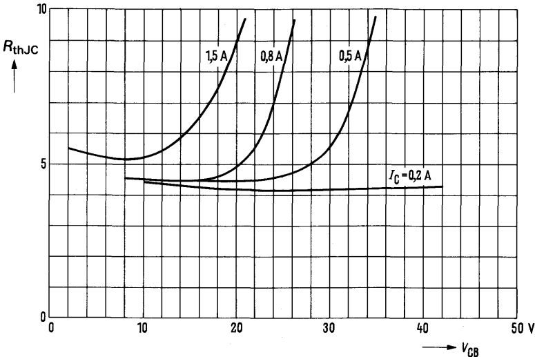
\frac{K}{W} Thermal resistance versus current and voltage R_{thJC} = f(V_{CB}) ( I_C = \text{parameter} )
