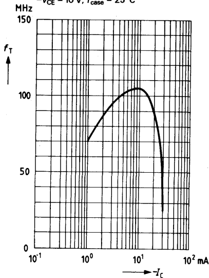
Transition frequency f_T = f(I_C) -V_{CE} = 10 \text{ V}; T_{case} = 25^{\circ}C
