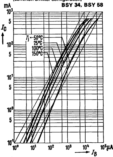
Collector current I_C = f(I_B) V_{CE} = 1\text{ V} (common emitter configuration)
