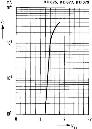
Collector current I_C = f(V_{BE}) -V_{CE} = 3 \text{ V}; T_{case} = 25^\circ\text{C} BD 675, BD 677, BD 679
