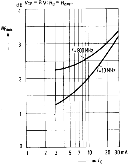
Min. noise figure NF_{min} = f(I_C)
