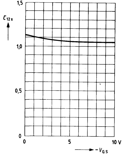
Reverse transfer capacitance
