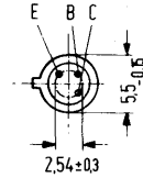
Dimensions in mm
