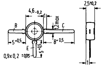
Approx. weight 0.25 g Dimensions in mm
