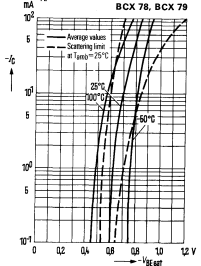
Base-emitter saturation voltage V_{BE\text{sat}} = f(I_C); T_{\text{amb}} = \text{parameter}; h_{FE} = 40
