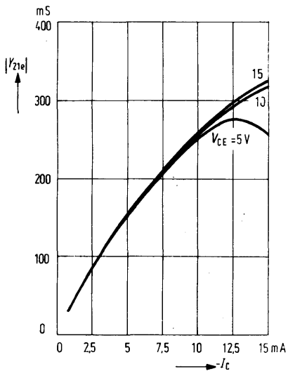
Short-circuit forward transfer admittance ( Y_{21a} ) = f(I_C) V_{CE} = \text{parameter}; f = 10.7 \text{ MHz}
