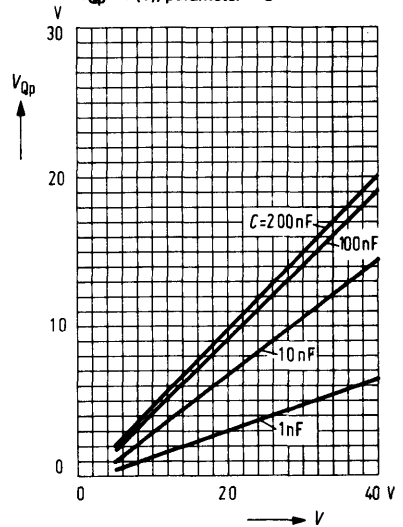
Peak output voltage V_{Op} = f(V); \text{parameter} = C
