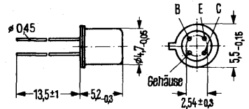
Approx. weight 0.4 g Dimensions in mm
