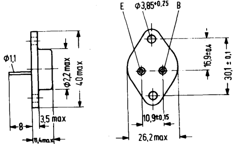
Approx. weight 18 g
