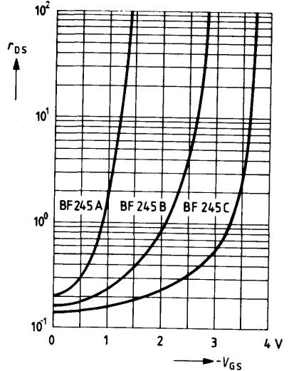
Dynamic drain-source resistance
