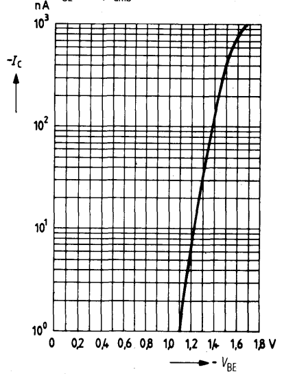
Collector current I_C = f(V_{BE}) V_{CE} = 2\text{ V}; T_{amb} = 25^\circ\text{C}
