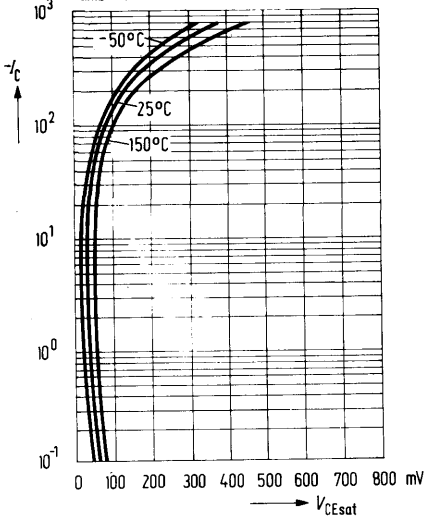
Collector-emitter saturation voltage V_{CEsat} = f(I_C); h_{FE} = 10; T_{amb} = \text{parameter}
