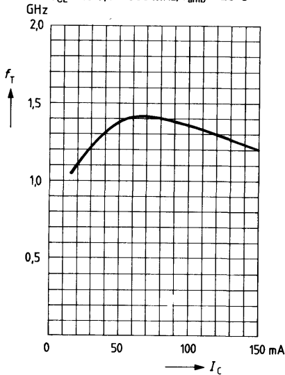
Transition frequency f_T = f(I_C) V_{CE} = 15 V, f = 500 MHz, T_{amb} = 25 °C
