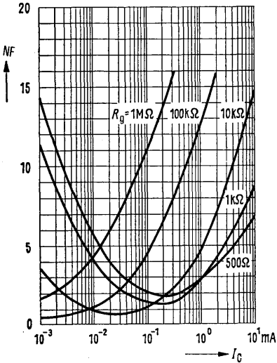
Noise figure NF = f(I_C) V_{CE} = 5 V; f = 1 kHz; T_{amb} = 25^\circ C
