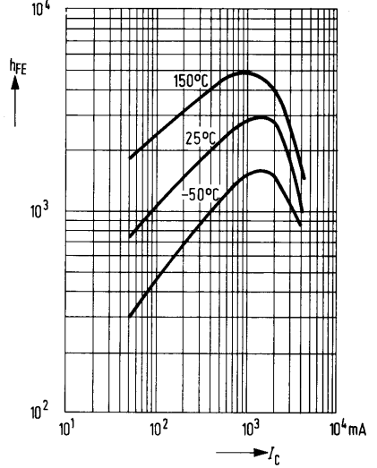
DC current gain h_{FE} = f(I_C) -V_{CE} = 3 \text{ V} BD 675, BD 677, BD 679
