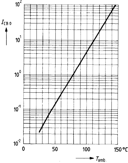
Collector cutoff current versus temperature I_{CB0} = f(T_{amb})
