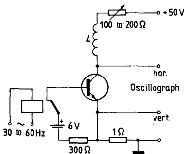
for V_{(BR)CE0}
