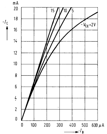
Collector current I_C = f(I_B) V_{CE} = \text{parameter}
