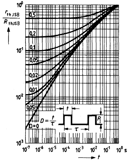
Pulse resistance D = \text{parameter}
