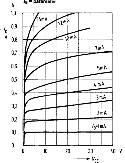
Output characteristics I_C = f(V_{CE}) I_B = \text{parameter}
