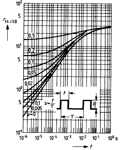
K Permissible pulse load
