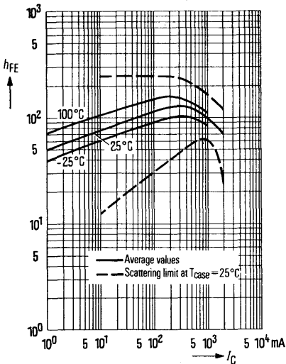
DC current gain h_{FE} = f(I_C) V_{CE} = 1 \text{ V}; T_{amb} = \text{parameter} (common emitter configuration)
