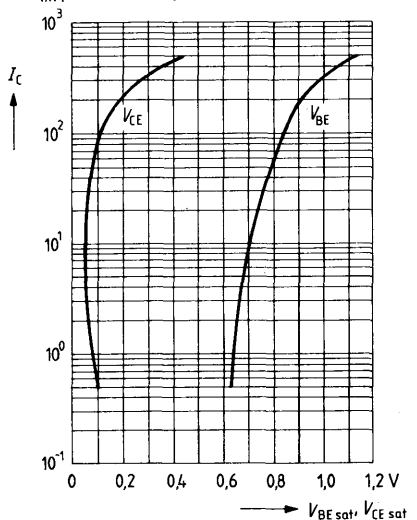
Saturation voltages V_{BEsat} = f(I_C), V_{CEsat} = f(I_C) mA h_{FE} = 10; T_{amb} = 25^\circ C
