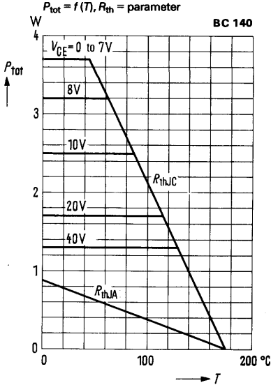
Total perm. power dissipation versus temperature P_{\text{Tot}} = f(T), R_{\text{th}} = \text{parameter}
