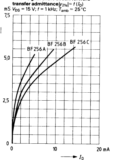
Small-signal short-circuit forward transfer admittance
