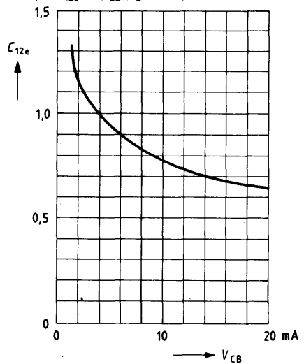
Reverse transfer capacitance C_{12e} = f(V_{\text{CB}}); I_C = 1 \text{ mA}; f = 1 \text{ MHz}
