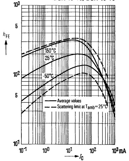
DC current gain h_{FE} = f(I_C) V_{CE} = 1 \text{ V} BSX 45-16, BSX 46-16
