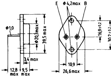
Approx. weight 18 g
