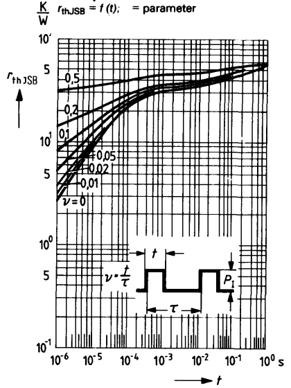
Perm. pulse load r_{th,JSB} = f(t); = \text{parameter}
