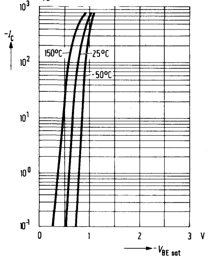
Base-emitter saturation voltage V_{BEsat} = f(I_C); T_{amb} = \text{parameter}; h_{FE} = 10
