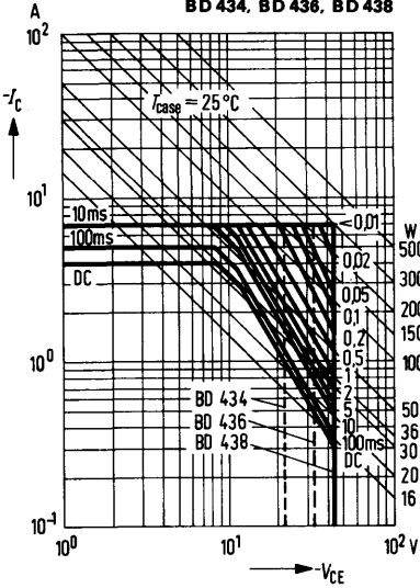
Permissible operating range I_C = f(V_{CE}); T_{case} = 25^\circ C, v = 0 BD 434, BD 436, BD 438
