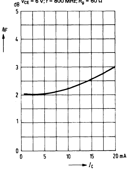
Noise figure NF = f(I_C) V_{CE} = 6 \text{ V}; f = 800 \text{ MHz}; R_g = 60 \Omega
