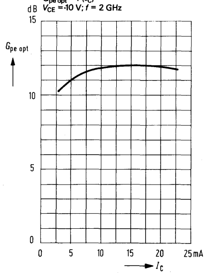
Max. power gain G_{pe\ opt} = f(I_C) V_{CE} = 10\ V; f = 2\ GHz
