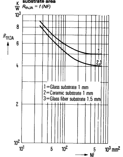
Thermal resistance versus substrate area R_{thJA} = f(NF)
