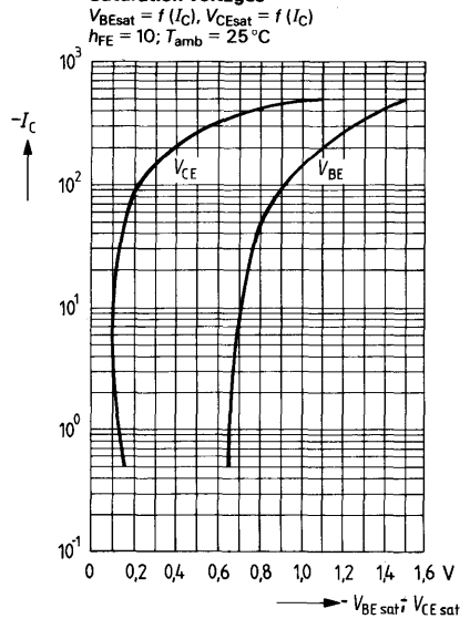
Saturation voltages
