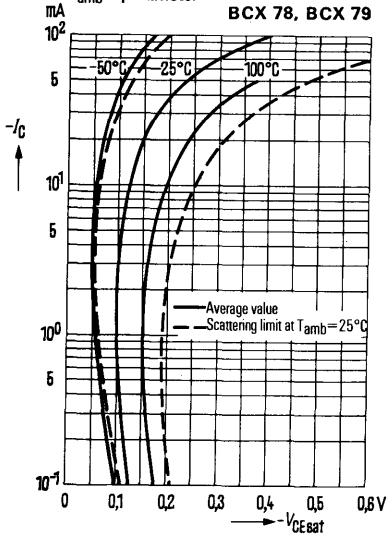
Collector-emitter saturation voltage V_{CE\text{sat}} = f(I_C); h_{FE} = 40; T_{\text{amb}} = \text{parameter}
