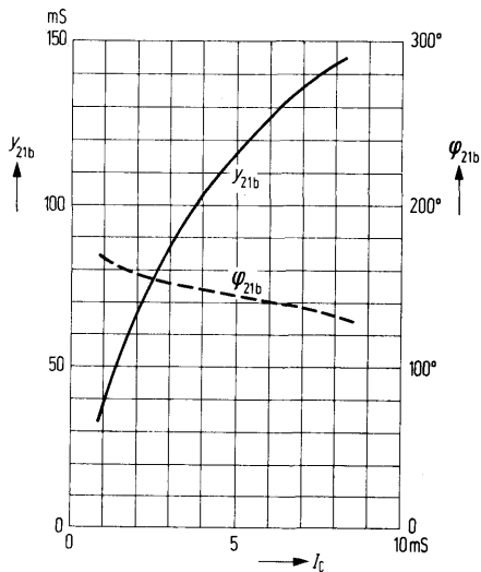
Short-circuit forward transfer admittance Y_{21b} = f(I_C) (common base configuration) -V_{CE} = 10 \text{ V}
