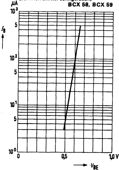
Input characteristics I_B = f(V_{BE}) V_{CE} = 5V (common emitter configuration)
