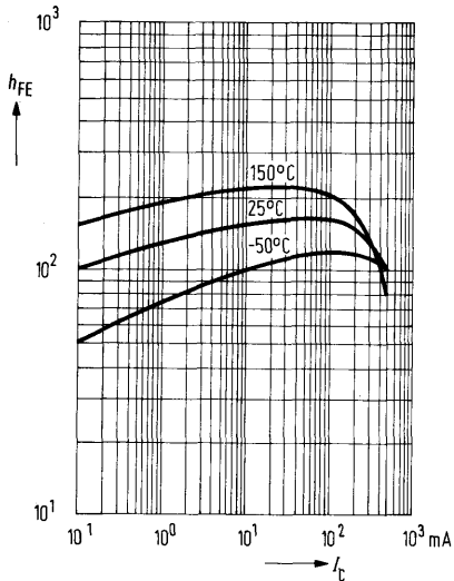
DC current gain h_{FE} = f(I_C) T_{\text{amb}} = \text{parameter}; V_{CE} = 1 \text{ V}
