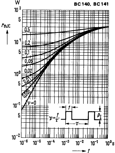
Permissible pulse load r_{\text{thJC}} = f(t); v = \text{parameter}
