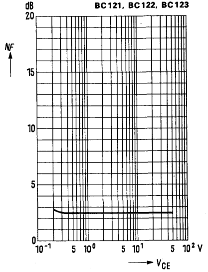
Noise figure NF = f(V_{CE}) (I_C = 0.2\text{ mA}, R_g = 2\text{ k}\Omega, f = 1\text{ kHz}) BC 121, BC 122, BC 123
