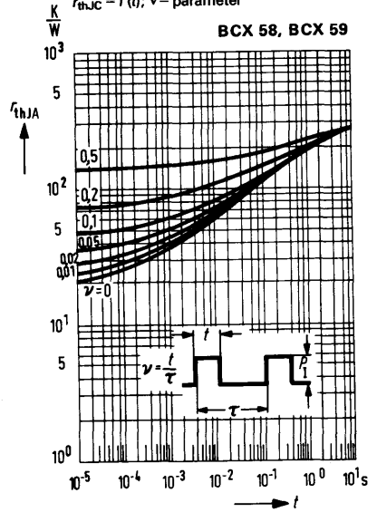
Permissible pulse load t_{thJC} = f(t); v = \text{parameter}
