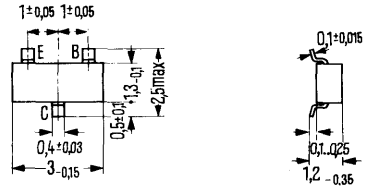
Approx. weight 0.02 g
