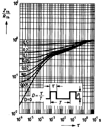
Permissible pulse load r_{thJA} = f(t)
