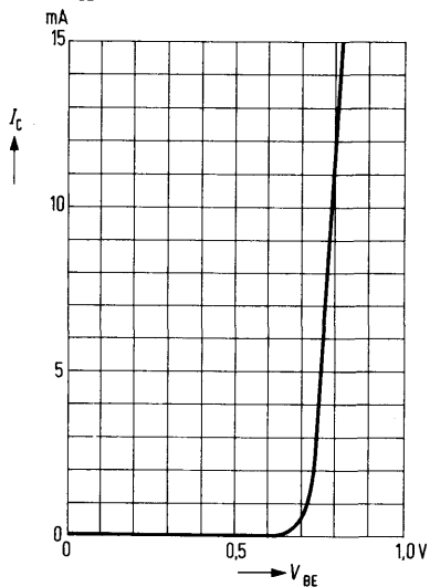
Input characteristic I_C = f(V_{BE})
