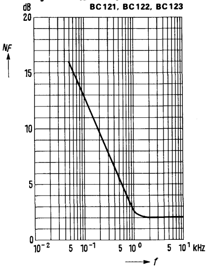
Noise figure NF = f(f) (R_g = 2\text{ k}\Omega, V_{CE} = 5\text{ V}, I_C = 0.2\text{ mA}) BC 121, BC 122, BC 123
