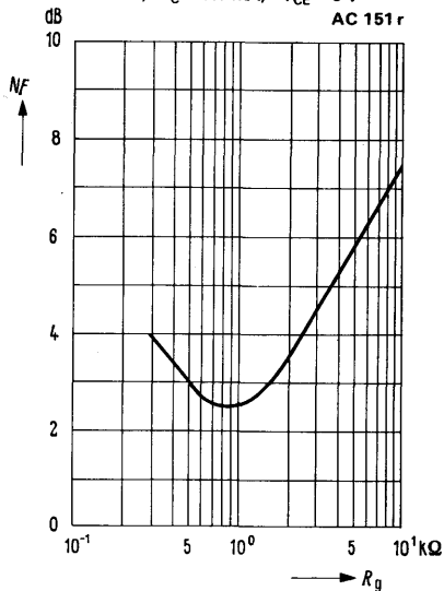
Noise figure versus internal resistance of generator NF = f(R_g)
