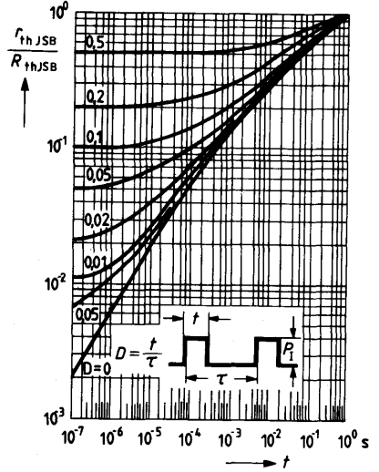
Pulse resistance \frac{r_{\text{thJSB}}}{R_{\text{thJSB}}} = f(t) D = parameter
