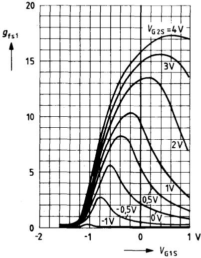
Gate 1 transadmittance g_{fs1} = f(V_{G1S})
