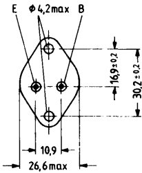
Approx. weight 18 g Dimensions in mm
