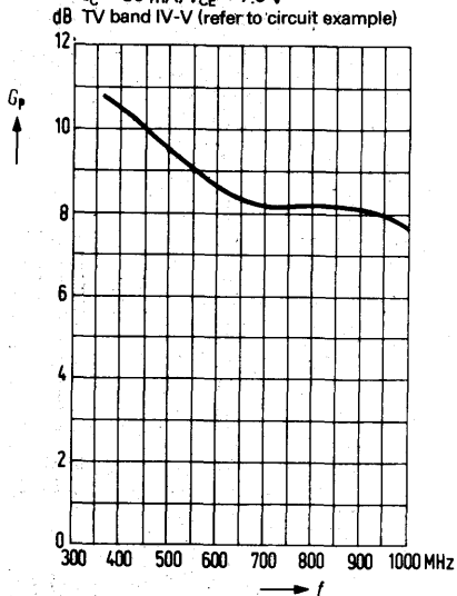
Power gain G_p = f(f) I_C = 80\text{ mA}; V_{CE} = 7.5\text{ V} TV band IV-V (refer to circuit example)
