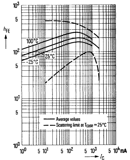
DC current gain h_{FE} = f(I_C) V_{CE} = 1 \text{ V}; T_{amb} = \text{parameter} (common emitter configuration)
