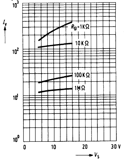
Valley point current I_v = f(V_S)
