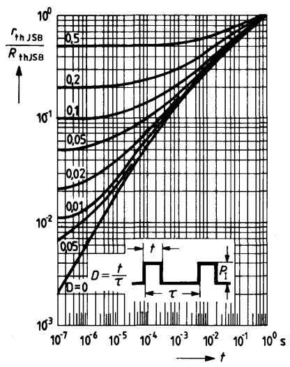
Perm. pulse load \frac{I_{thJSB}}{R_{thJSB}} = f(t) D = parameter
