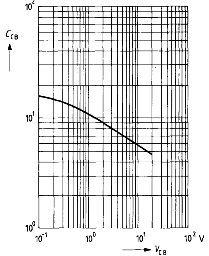
Collector-base capacitance C_{CB} = f(V_{CB}); T_{amb} = 25^\circ C
