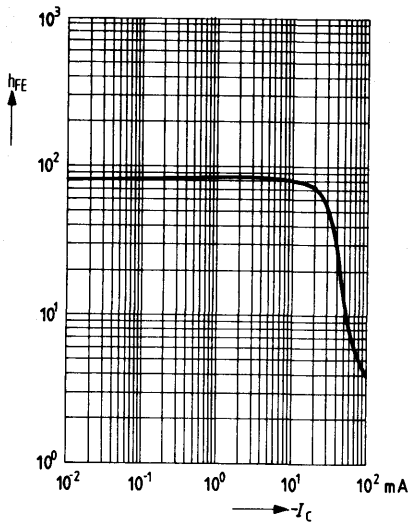
DC current gain h_{FE} = f(I_C) -V_{CE} = 10 \text{ V}; T_{case} = 25^{\circ}C
