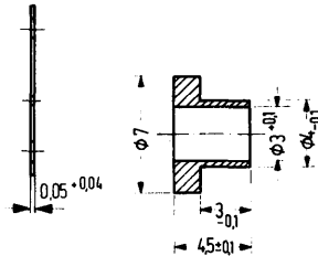
Insulating nipple
