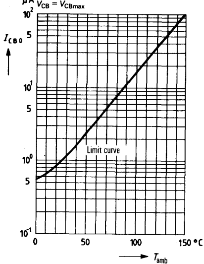
Collector cutoff current versus temperature I_{CBO} = f(T_{amb}) V_{CB} = V_{CBmax}
