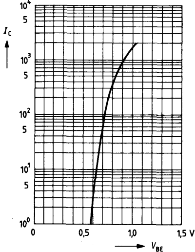
Collector current I_C = f(V_{BE}) V_{CE} = 1\text{ V}; T_{amb} = 25^\circ\text{C}
