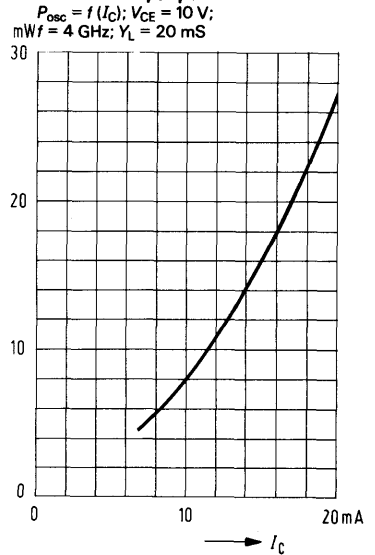
Oscillator output power
