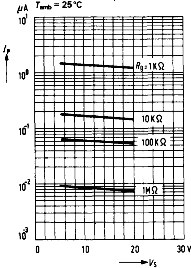
Peak point current I_p = f(V_S)
