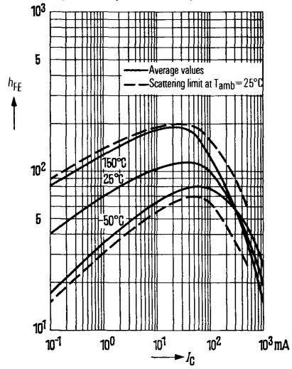
DC current gain h_{FE} = f(I_C) V_{CE} = 1 \text{ V} BSX 45-10, BSX 46-10, BSX 47-10
