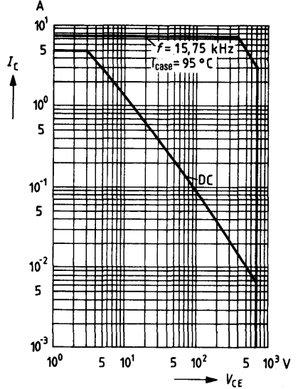
Permissible operating range I_C = f(V_{CE}); T_{case} = 95^\circ\text{C}
