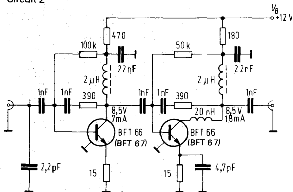
Circuit 2
