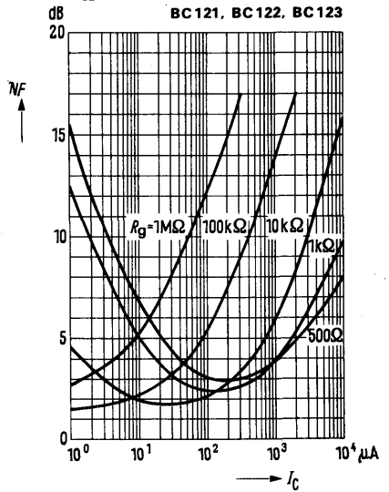
Noise figure NF = f(I_C) (V_{CE} = 5\text{ V}; f = 1\text{ kHz}, T_{amb} = 25^\circ\text{C}) BC 121, BC 122, BC 123
