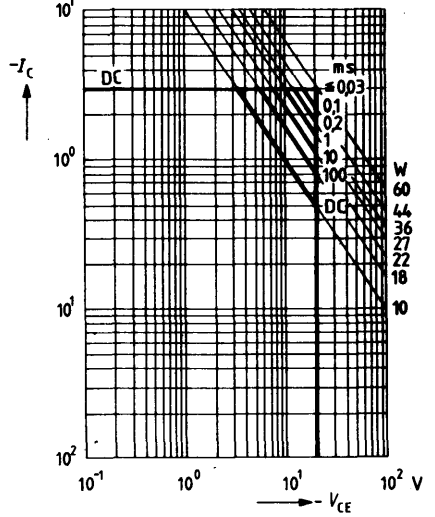
Permissible operating range I_C = f(V_{CE}) D = 0; T_{case} = 25^\circ\text{C}
