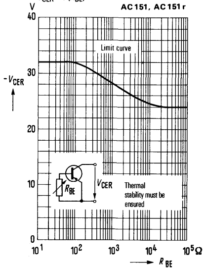
Collector-emitter voltage
