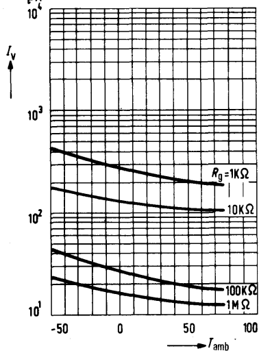
Valley point current I_v = f(T_{amb})
