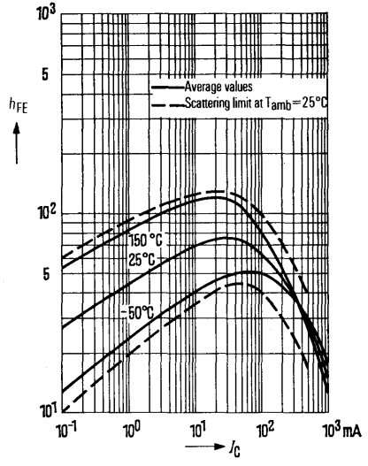
DC current gain h_{FE} = f(I_C) V_{CE} = 1 \text{ V} BSX 45-6, BSX 46-6, BSX 47-6
