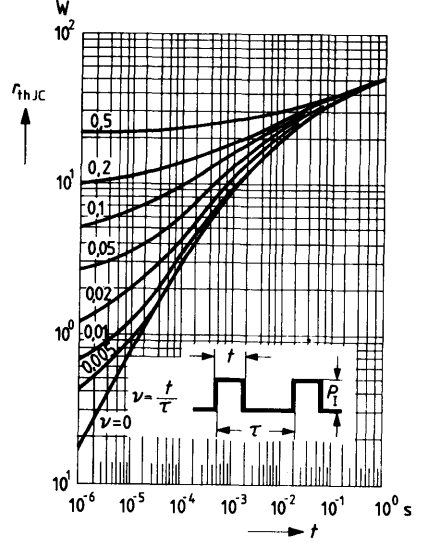
Permissible pulse load r_{thJC} = f(t) v = \text{parameter}
