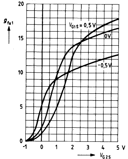
Gate 2 transadmittance g_{fs1} = f(V_{G2S})
