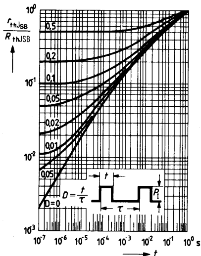
Perm. pulse load r_{thJSB} = f(t) D = \text{parameter} R_{thJSB}
