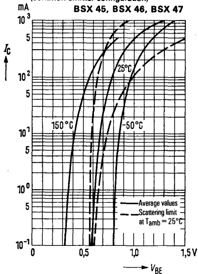
Collector current I_C = f(V_{BE}) V_{CE} = 1\text{ V}; T_{amb} = \text{parameter} (common emitter configuration)
