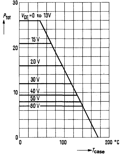
Permissible total power dissipation versus temperature P_{tot} = f(T_{case}) ; W ( V_{CE} = \text{parameter} )
