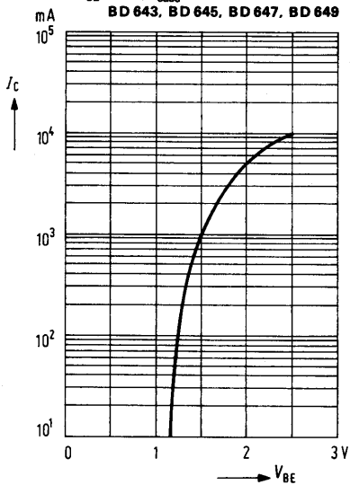
Collector current I_C = f(V_{BE}) V_{CE} = 3\text{ V}; T_{case} = 25^\circ\text{C} BD 643, BD 645, BD 647, BD 649
