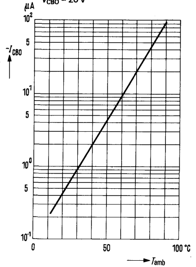
Collector cutoff current versus temperature I_{CBO} = f(T_{amb}) ; -V_{CBO} = 20\text{ V}
