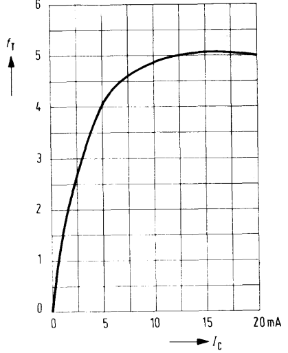
Transition frequency f_T = f(I_C) 6GHz V_{CE} = 8V; f = 200\text{ MHz}
