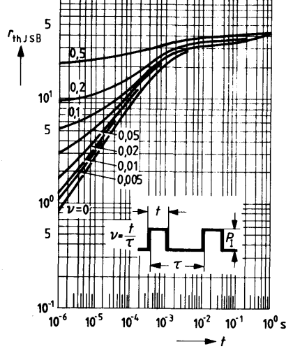
Permissible pulse load r_{thSB} = f(t)
