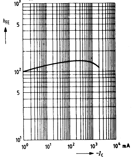
DC current gain h_{FE} = f(I_C) -V_{CE} = 1\text{ V}, T_{amb} = 25^\circ\text{C}
