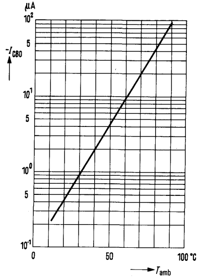
Collector cutoff current versus temperature
